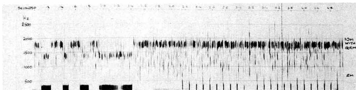
Fig 10. (a) (top) Simultaneous recordings of ZE2JV 28 and 144MHz beacons as received by SV11DH in Athens at 1755gmt on 13 February 1979. (b) (below) Enlargement of part of the recording showing coinciding pulses on 28 and 144MHz
