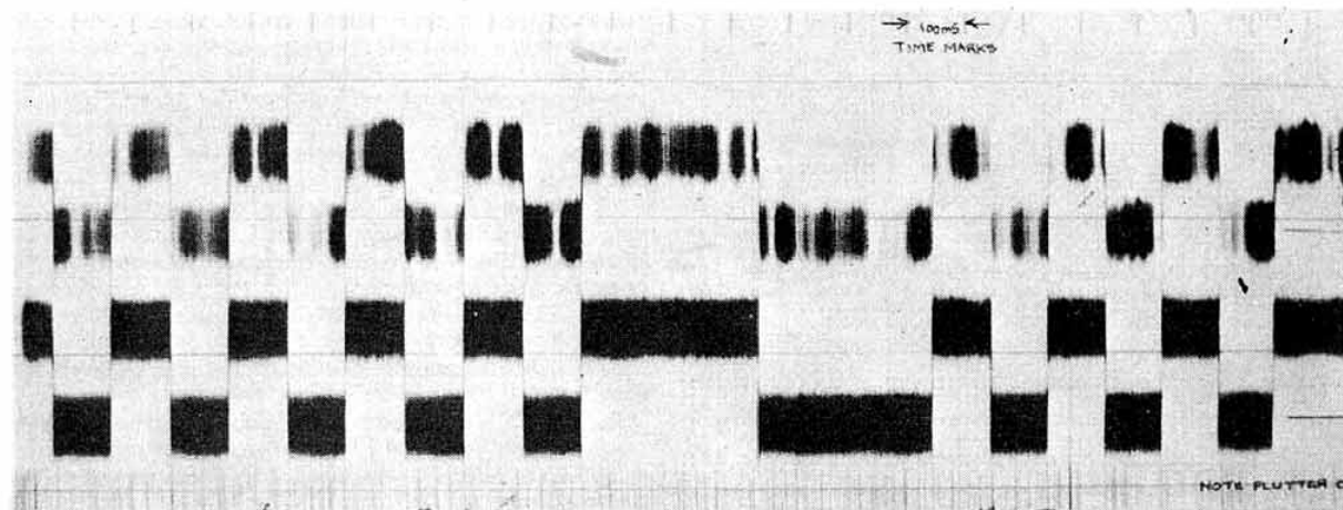
Fig 8. The letters 5B of 5B4CY as received by ZS6PW at 1845gmt on 30 January 1979 simultaneously on 50.498 and 28.220MHz. Note that the 50MHz pulse is 2ms behind the 28MHz pulse, which is a function of the keyer
