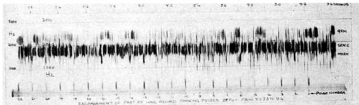
Fig 10. (a) (top) Simultaneous recordings of ZE2JV 28 and 144MHz beacons as received by SV11DH in Athens at 1755gmt on 13 February 1979. (b) (below) Enlargement of part of the recording showing coinciding pulses on 28 and 144MHz
